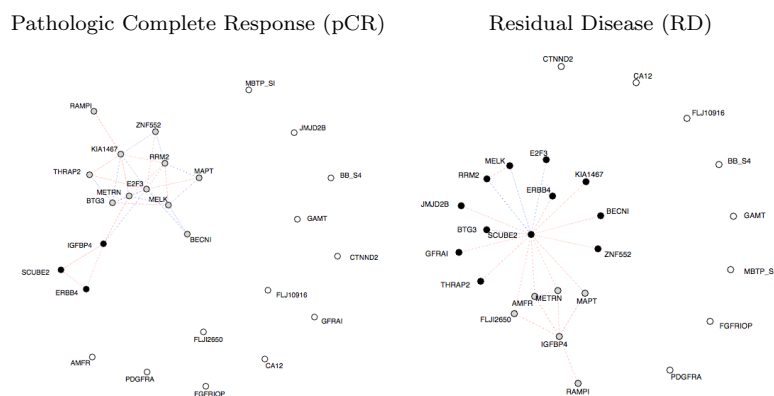
FIG 6. Graphs of conditional dependencies among the 26 genes selected by [23] on patients with pathologic complete response or residual disease with medium regularization as presented in Figure 3 of [1].
