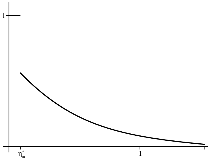
Figure 1.1: The typical graph of a majorant of \mathbf{AC} function.
