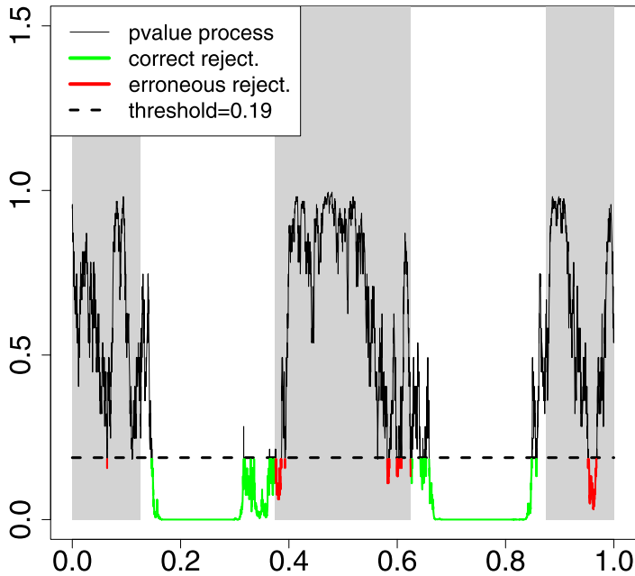
Figure 2. Several plots versus t \in [0, 1] . Top left: \lambda(t) (solid) and \lambda_0 (dashed). Top right: q_{\sigma(k)}(X) and \alpha \sum_{\ell=0}^k w_\ell in function of \sum_{\ell=0}^k w_\ell , for k = 1, \dots, m . Bottom: p -value process p_t(X) defined by (19). \eta = 0.015 , \alpha = 0.4 . The grey areas indicate regions where the null hypotheses are true.
