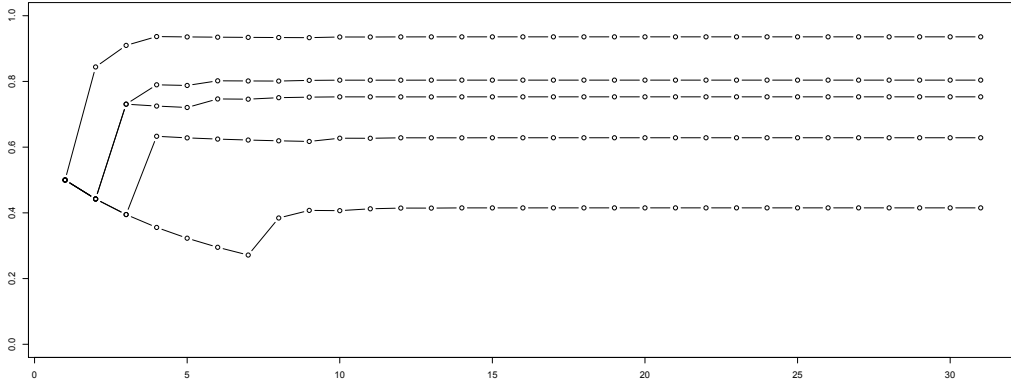
FIGURE 3. Plot of five realizations of the process (2 \arctan(y_n/x_n)/\pi) in the case in which we are considering Y_1 Y_2 \dots Y_n , so the process is not Markovian. It converges very quickly to a random limit point. We will see that in this particular case the law of this invariant limit point is the invariant measure that appears in Fig. 2, but this is just an artefact of the symmetries of this specific example.
